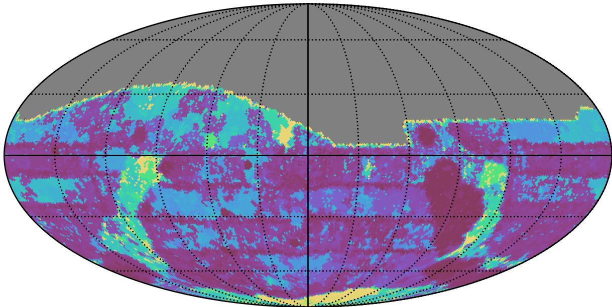
too_elab_r16_d2_giz_v3.4_10yrs All sky g band: Max Inter-Night Gap
