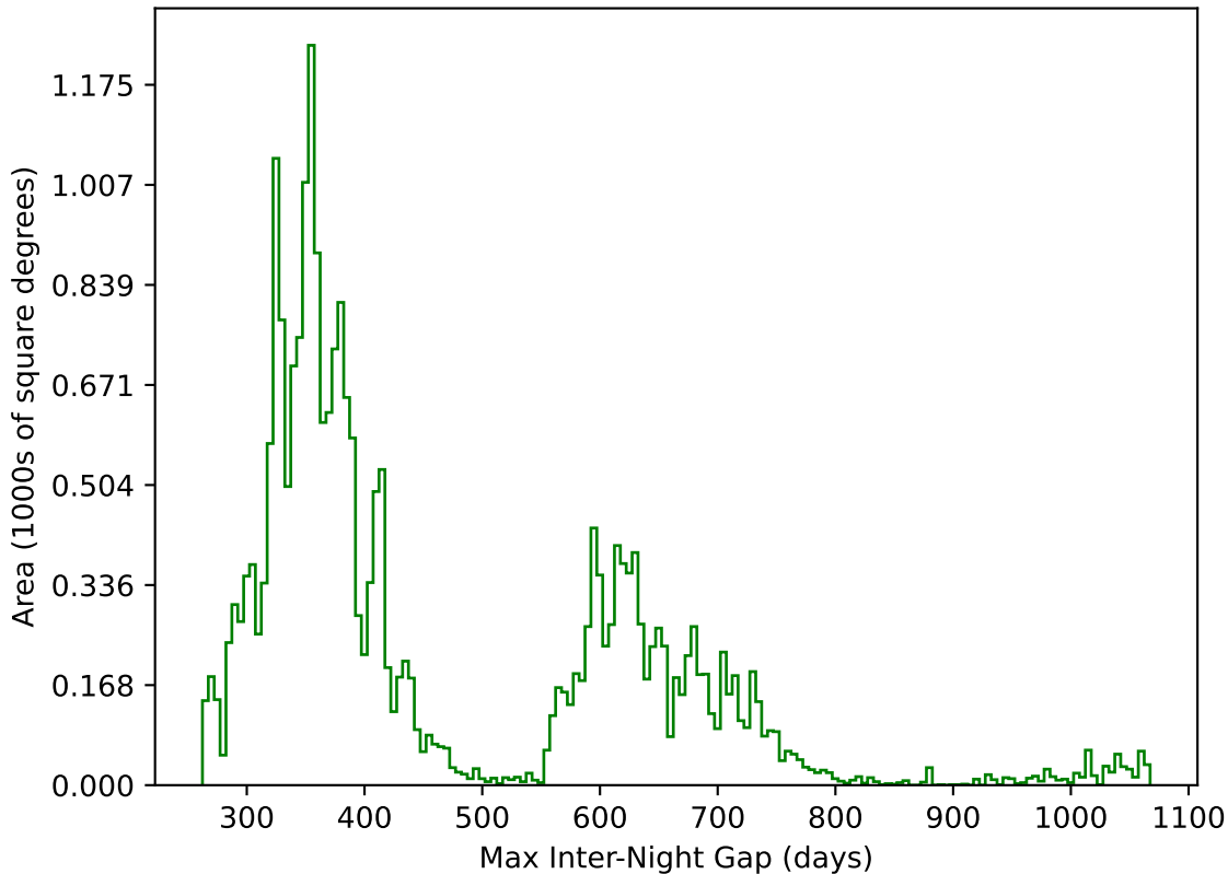
too_elab_r16_d2_giz_v3.4_10yrs All sky g band: Max Inter-Night Gap
