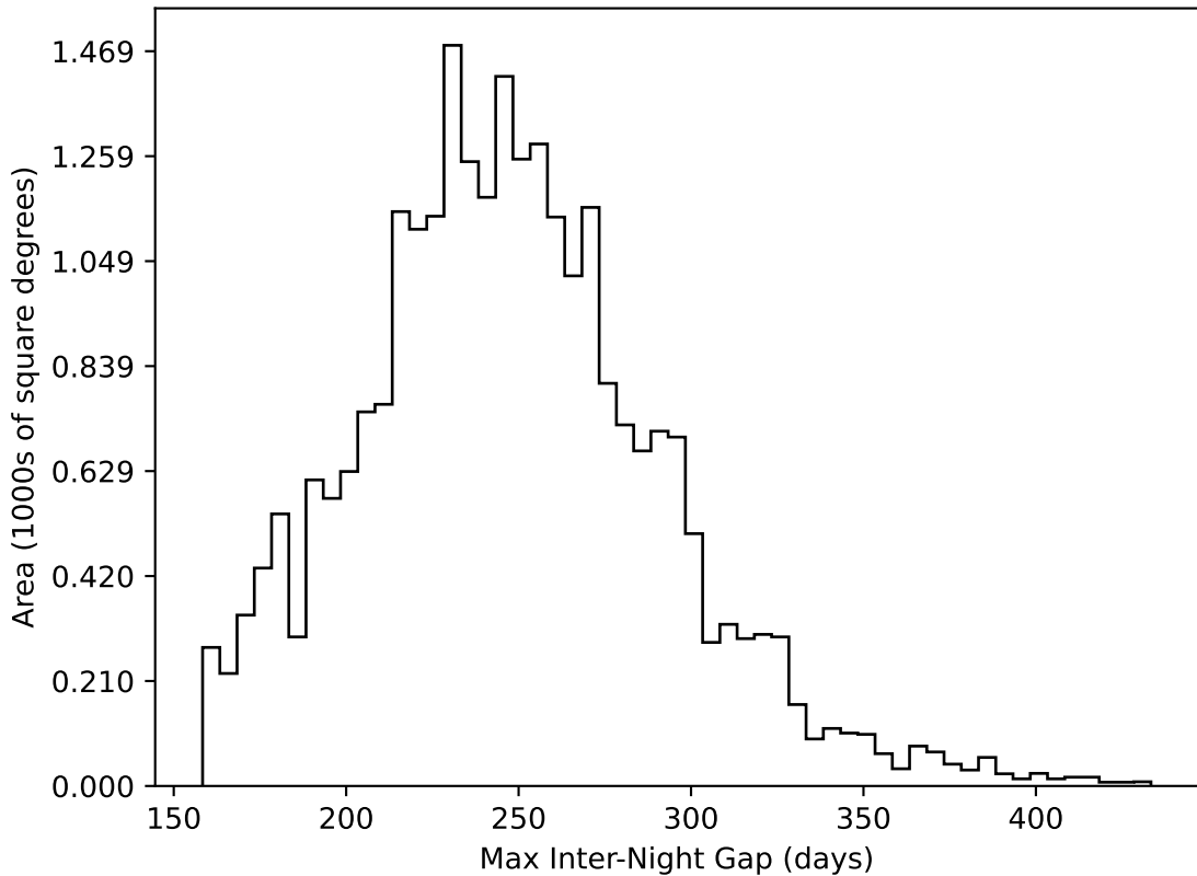
too_elab_r16_d2_giz_v3.4_10yrs All sky all bands: Max Inter-Night Gap
