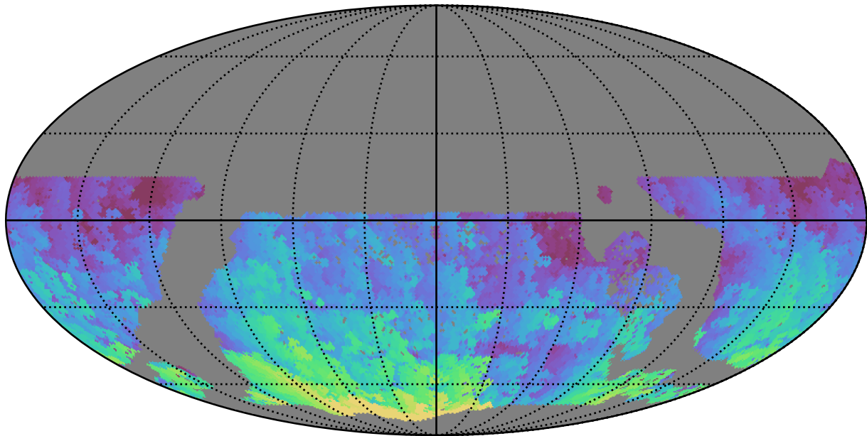
too_elab_r16_d2_giz_v3.4_10yrs WFD u band: Max HA
