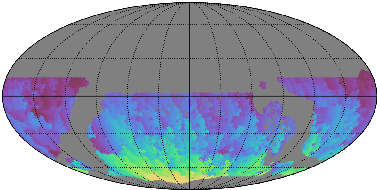
too_elab_r16_d2_giz_v3.4_10yrs WFD r band: Max HA
