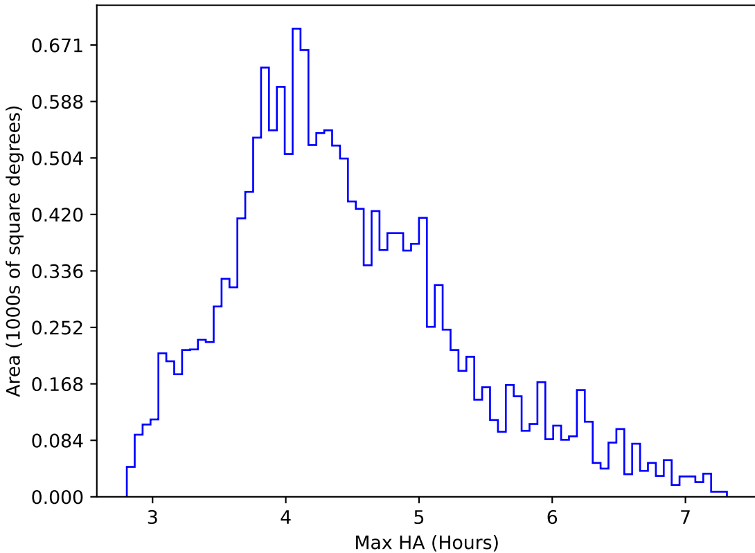
too_elab_r16_d2_giz_v3.4_10yrs WFD r band: Max HA
