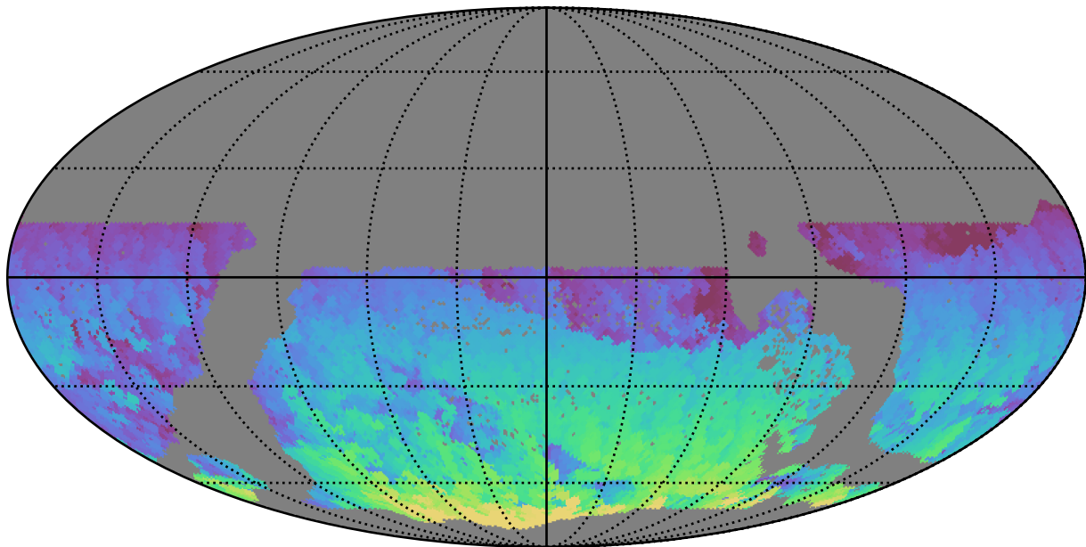
too_elab_r16_d2_giz_v3.4_10yrs WFD i band: Max HA
