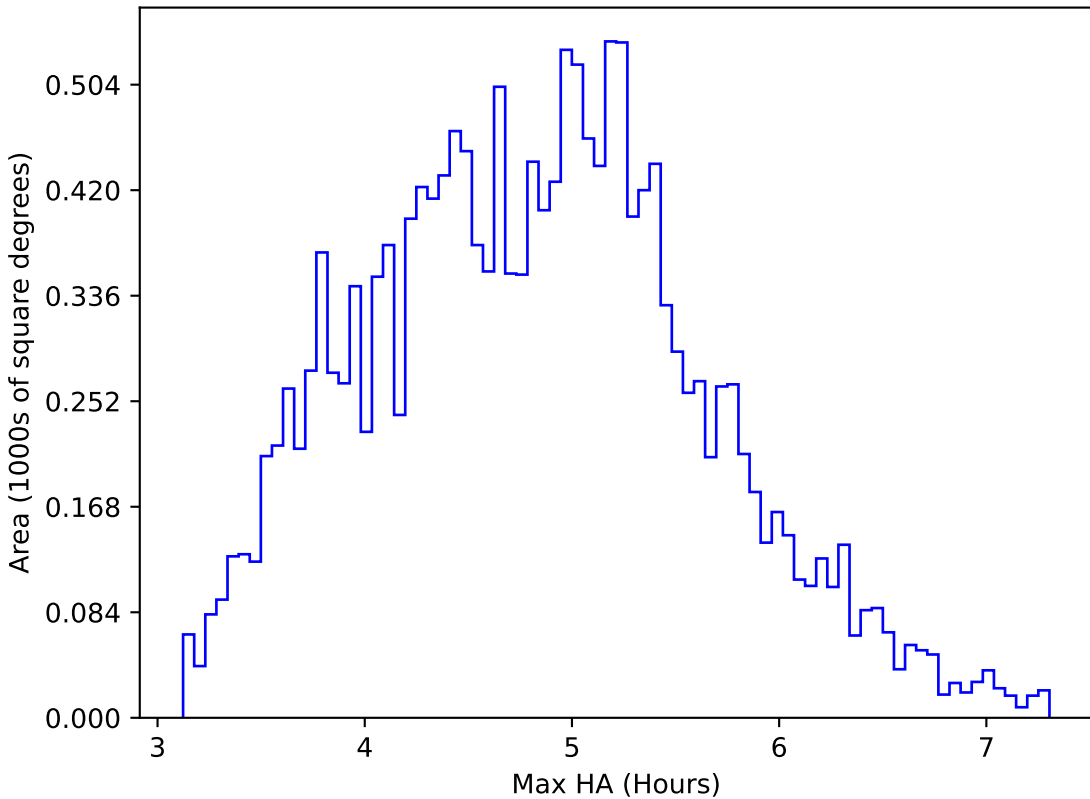
too_elab_r16_d2_giz_v3.4_10yrs WFD i band: Max HA
