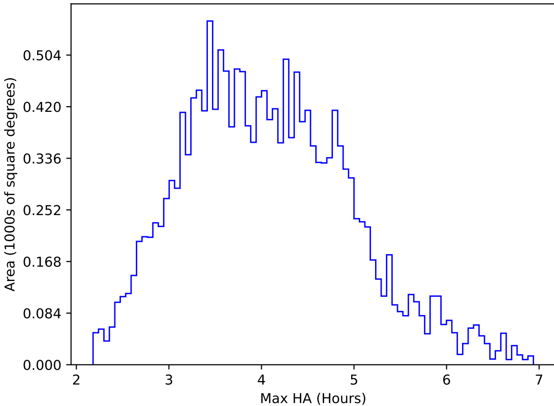
too_elab_r16_d2_giz_v3.4_10yrs WFD g band: Max HA
