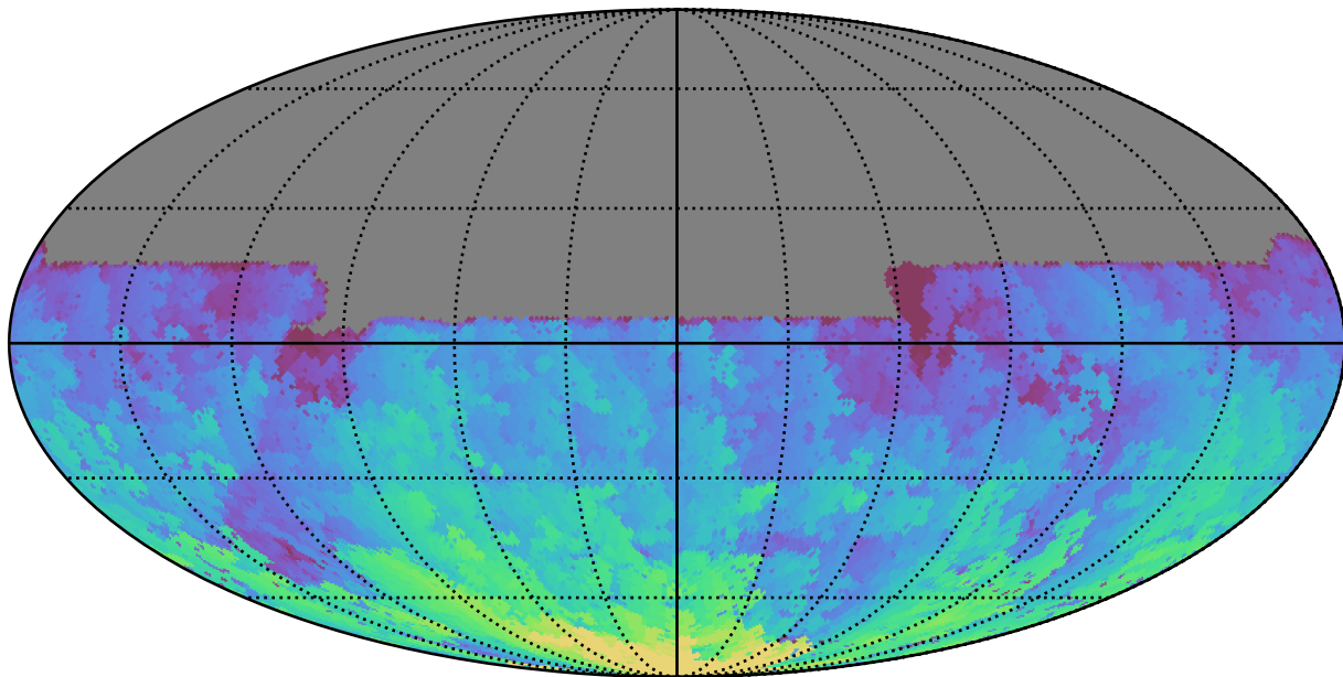
too_elab_r16_d2_giz_v3.4_10yrs All sky u band: Max HA
