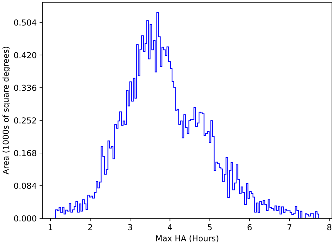
too_elab_r16_d2_giz_v3.4_10yrs All sky u band: Max HA
