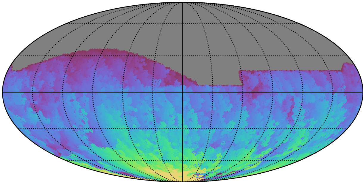
too_elab_r16_d2_giz_v3.4_10yrs All sky r band: Max HA
