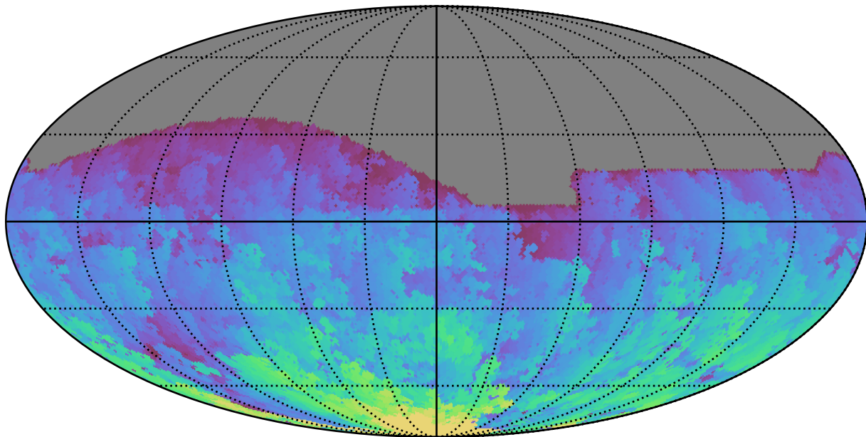
too_elab_r16_d2_giz_v3.4_10yrs All sky g band: Max HA
