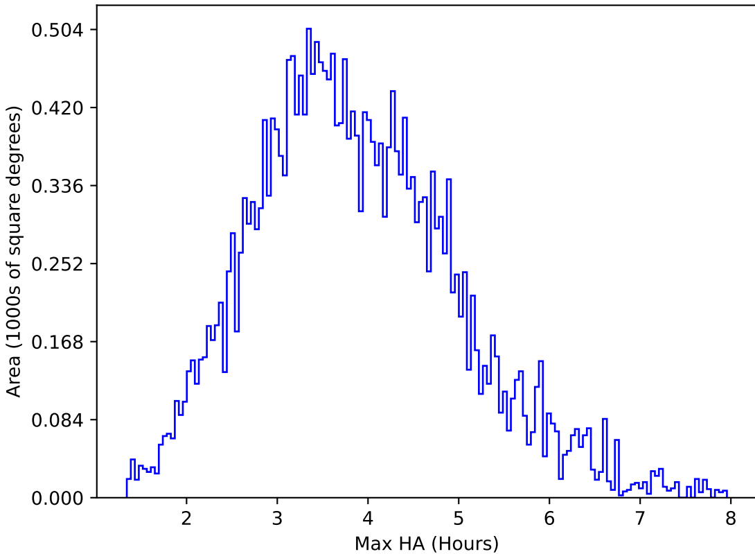
too_elab_r16_d2_giz_v3.4_10yrs All sky g band: Max HA
