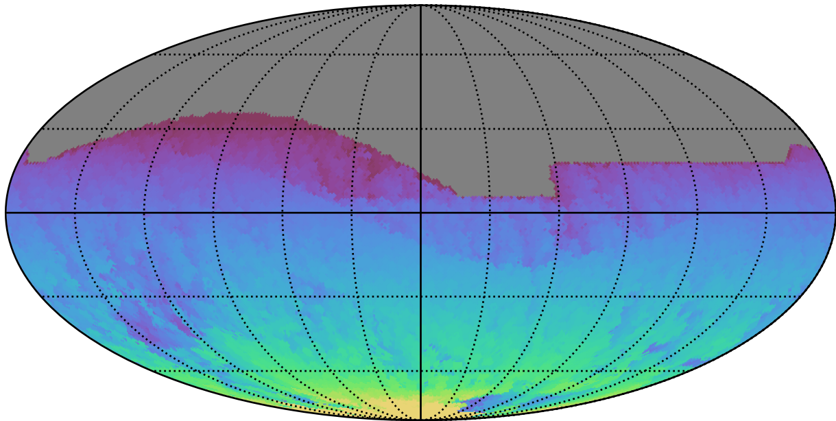
too_elab_r16_d2_giz_v3.4_10yrs All sky all bands: Max HA
