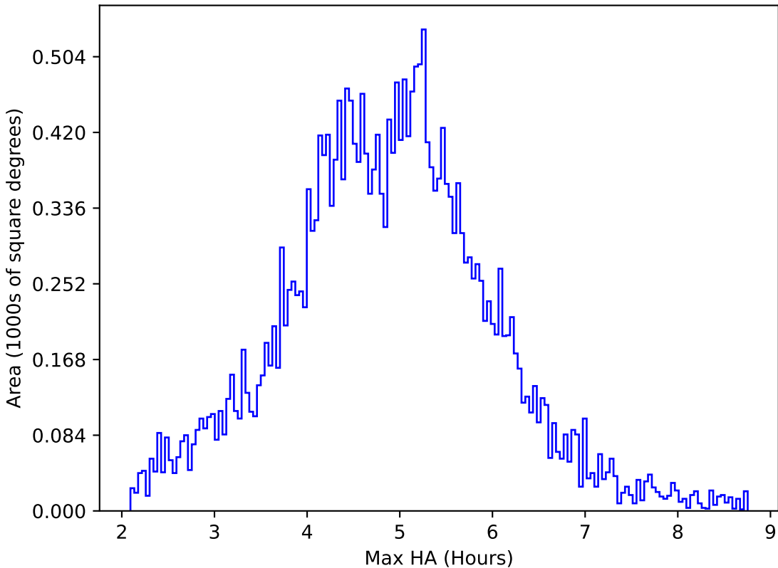
too_elab_r16_d2_giz_v3.4_10yrs All sky all bands: Max HA
