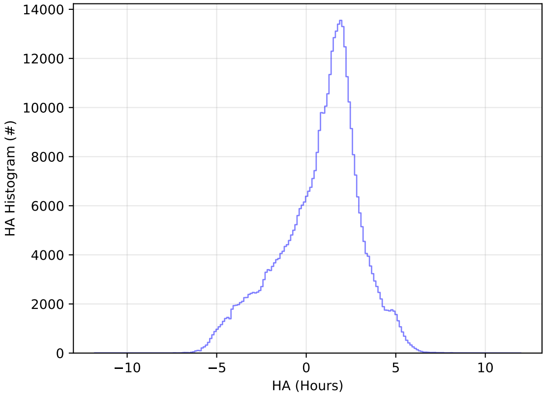
too_elab_r16_d2_giz_v3.4_10yrs WFD z band: HA Histogram
