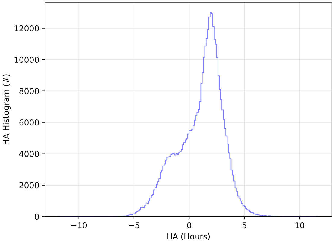
too_elab_r16_d2_giz_v3.4_10yrs WFD y band: HA Histogram
