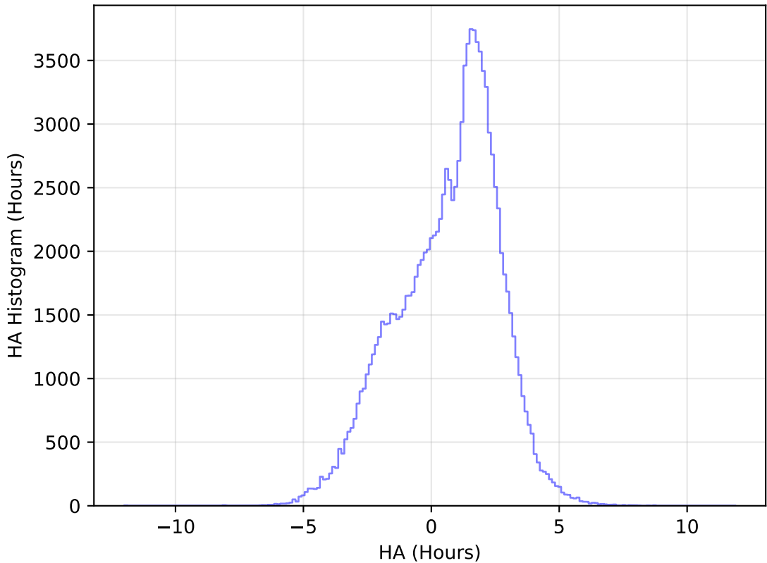
too_elab_r16_d2_giz_v3.4_10yrs WFD u band: HA Histogram
