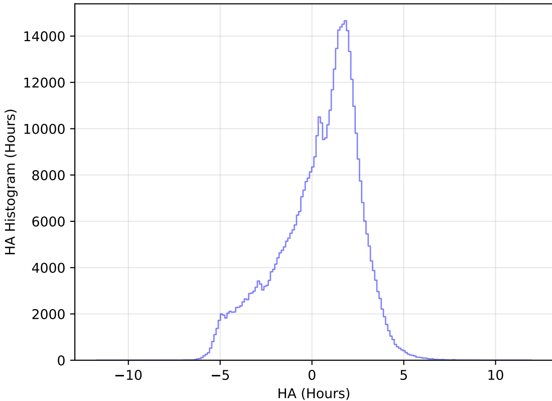
too_elab_r16_d2_giz_v3.4_10yrs WFD r band: HA Histogram
