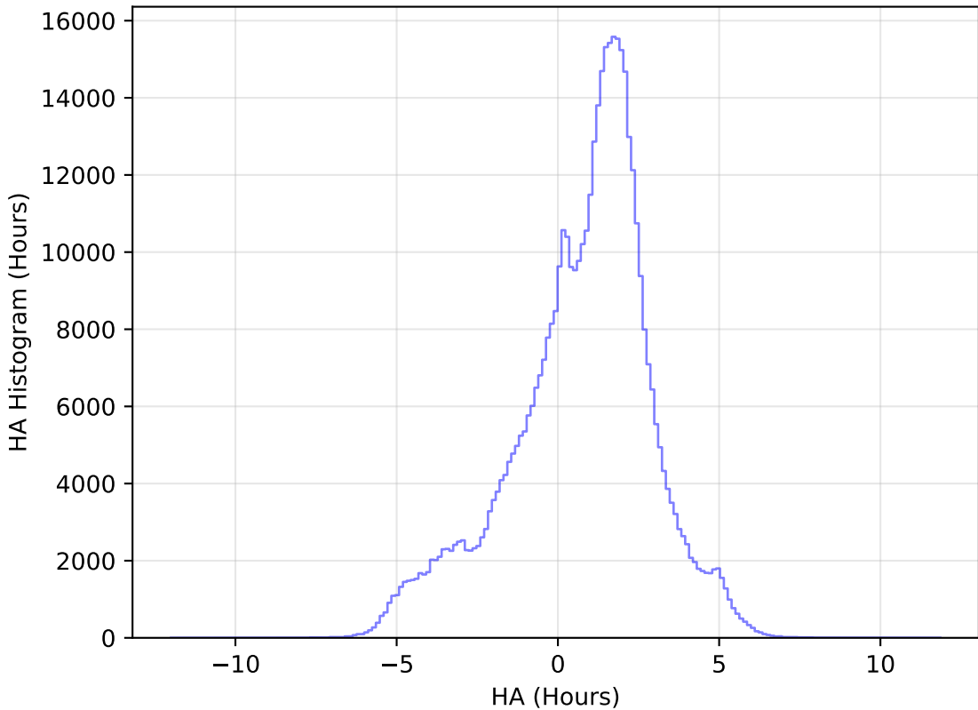
too_elab_r16_d2_giz_v3.4_10yrs WFD i band: HA Histogram
