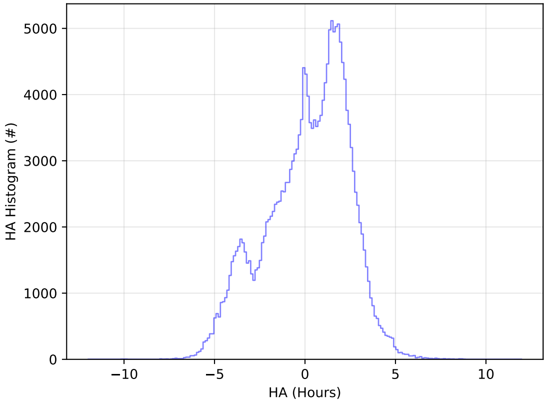
too_elab_r16_d2_giz_v3.4_10yrs WFD g band: HA Histogram
