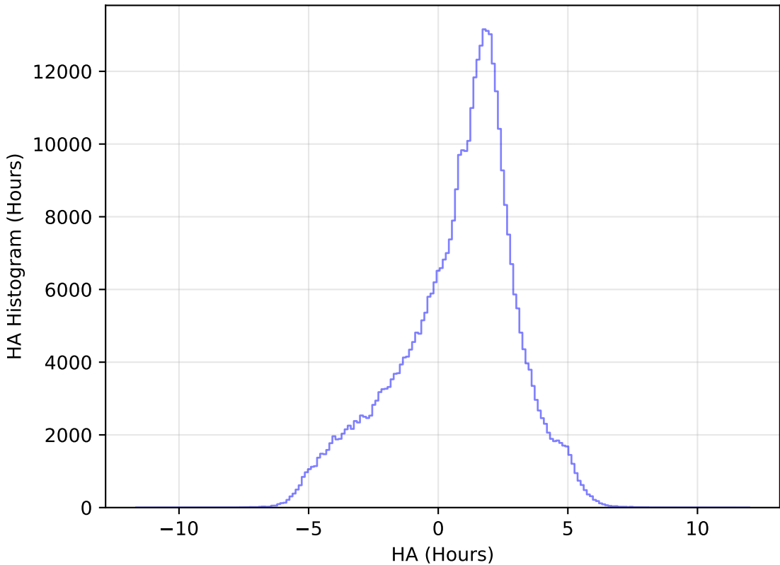
too_elab_r16_d2_giz_v3.4_10yrs All sky z band: HA Histogram
