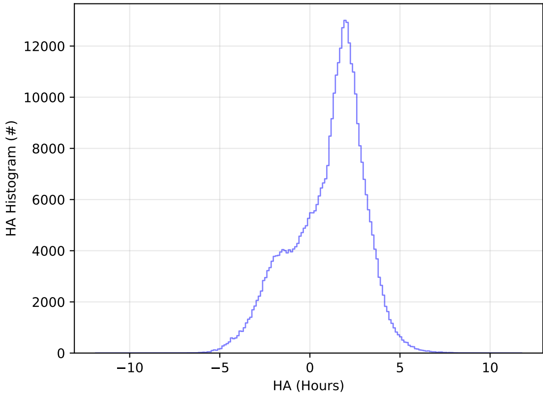
too_elab_r16_d2_giz_v3.4_10yrs All sky y band: HA Histogram
