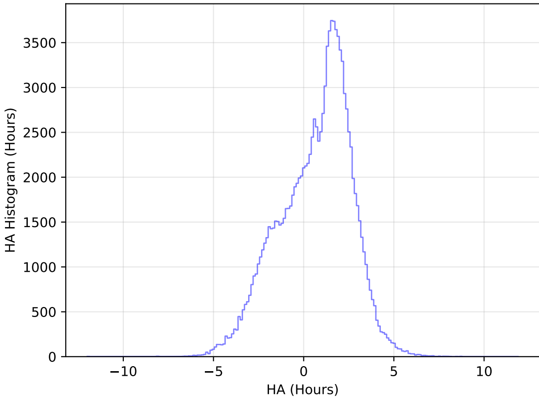
too_elab_r16_d2_giz_v3.4_10yrs All sky u band: HA Histogram
