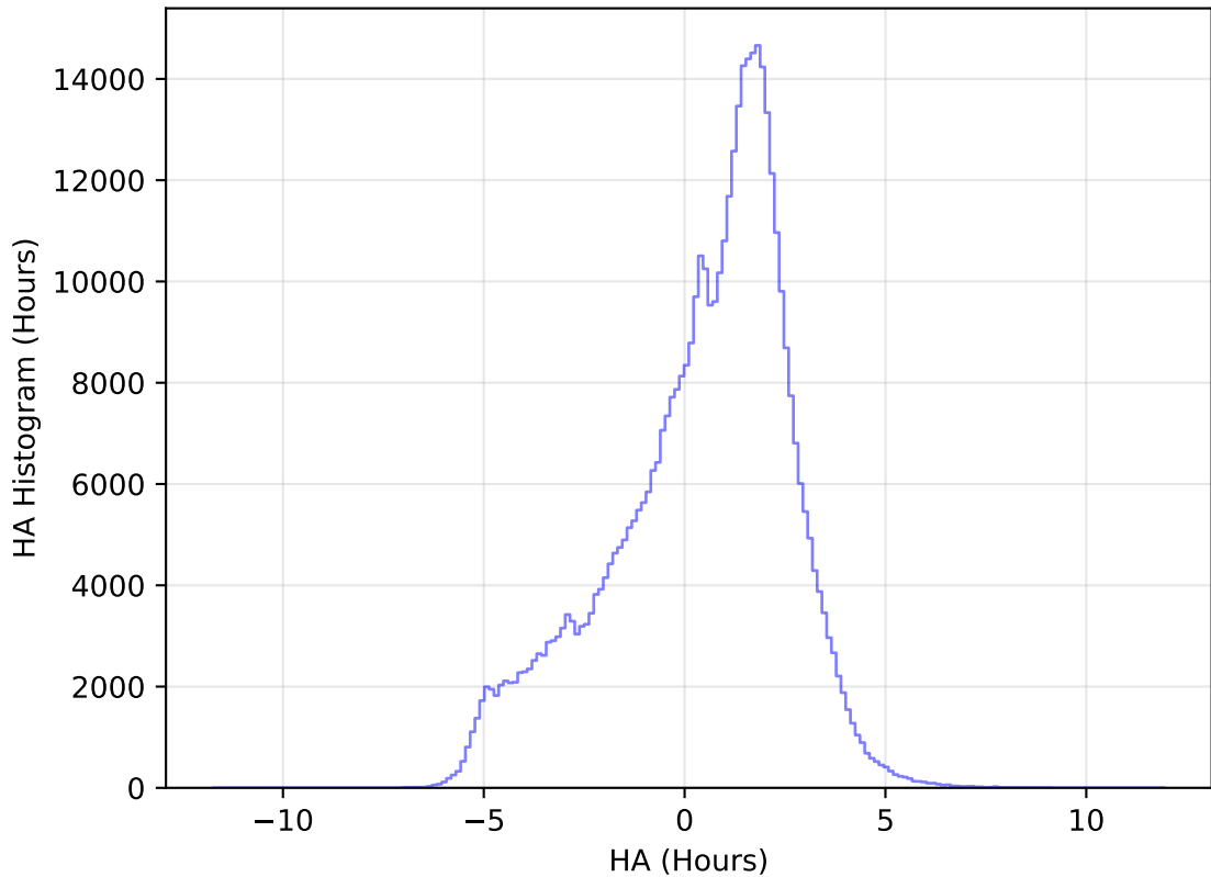
too_elab_r16_d2_giz_v3.4_10yrs All sky r band: HA Histogram
