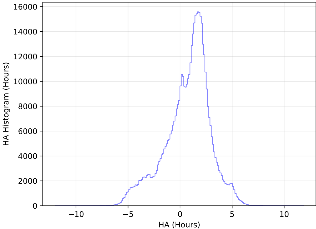
too_elab_r16_d2_giz_v3.4_10yrs All sky i band: HA Histogram
