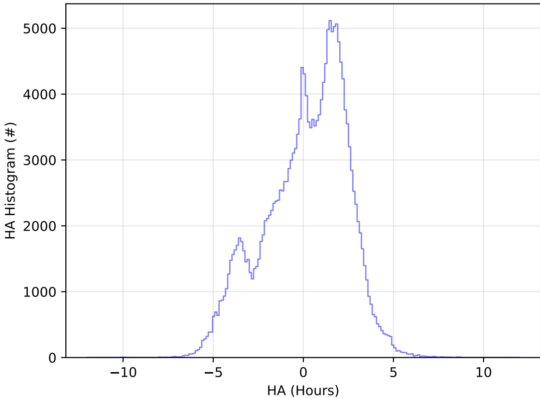
too_elab_r16_d2_giz_v3.4_10yrs All sky g band: HA Histogram
