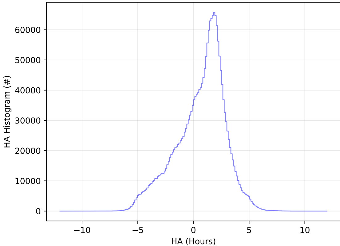
too_elab_r16_d2_giz_v3.4_10yrs All sky all bands: HA Histogram
