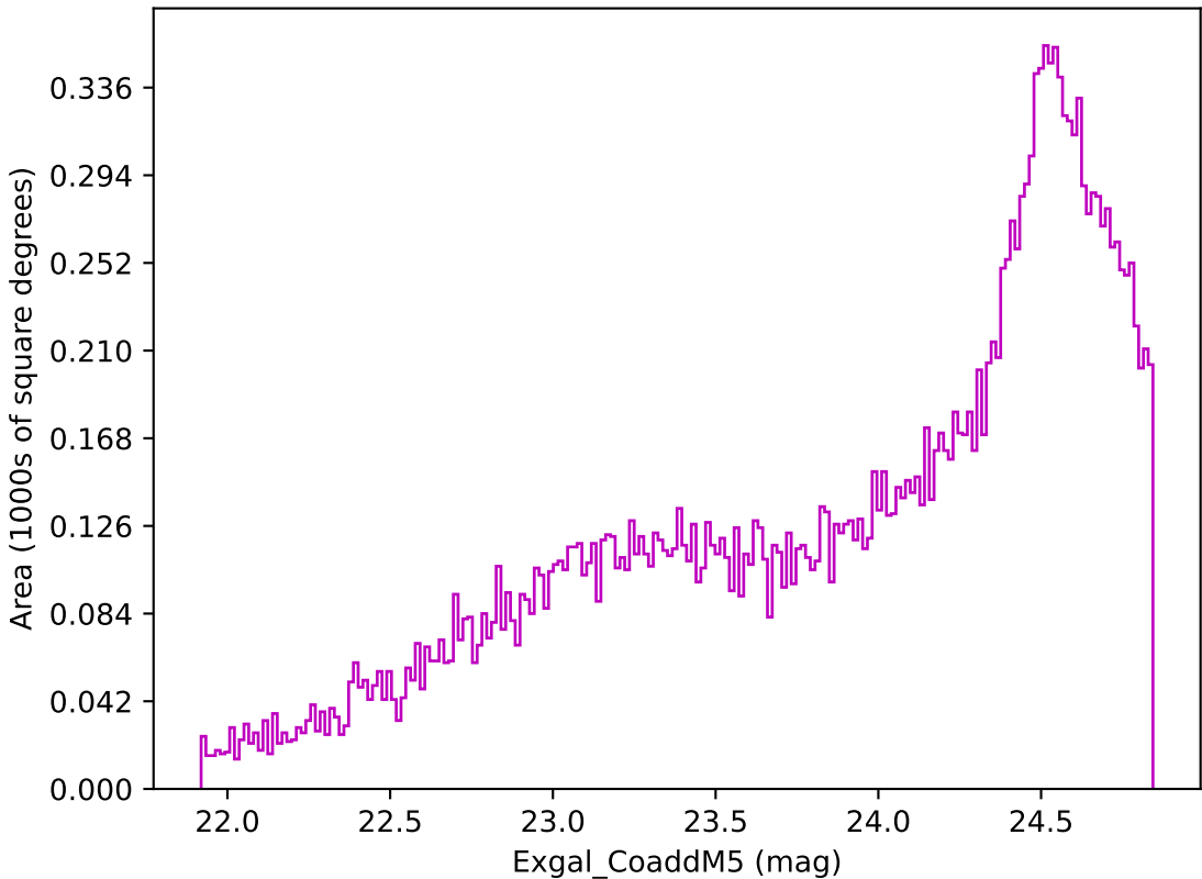
too_elab_r16_d2_giz_v3.4_10yrs Yr 3-4 z band: Exgal_CoaddM5
