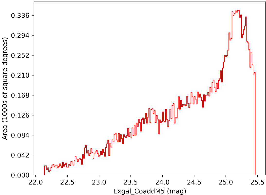
too_elab_r16_d2_giz_v3.4_10yrs Yr 3-4 i band: Exgal_CoaddM5
