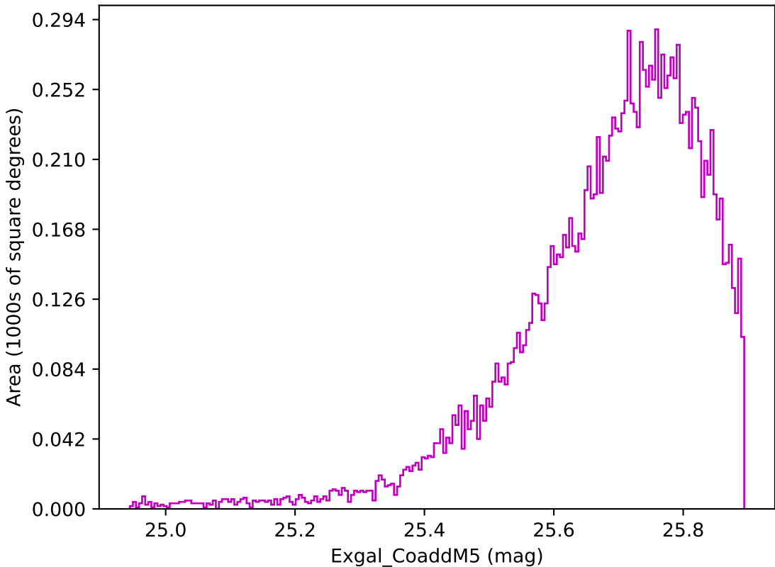
too_elab_r16_d2_giz_v3.4_10yrs WFD z band: Exgal_CoaddM5
