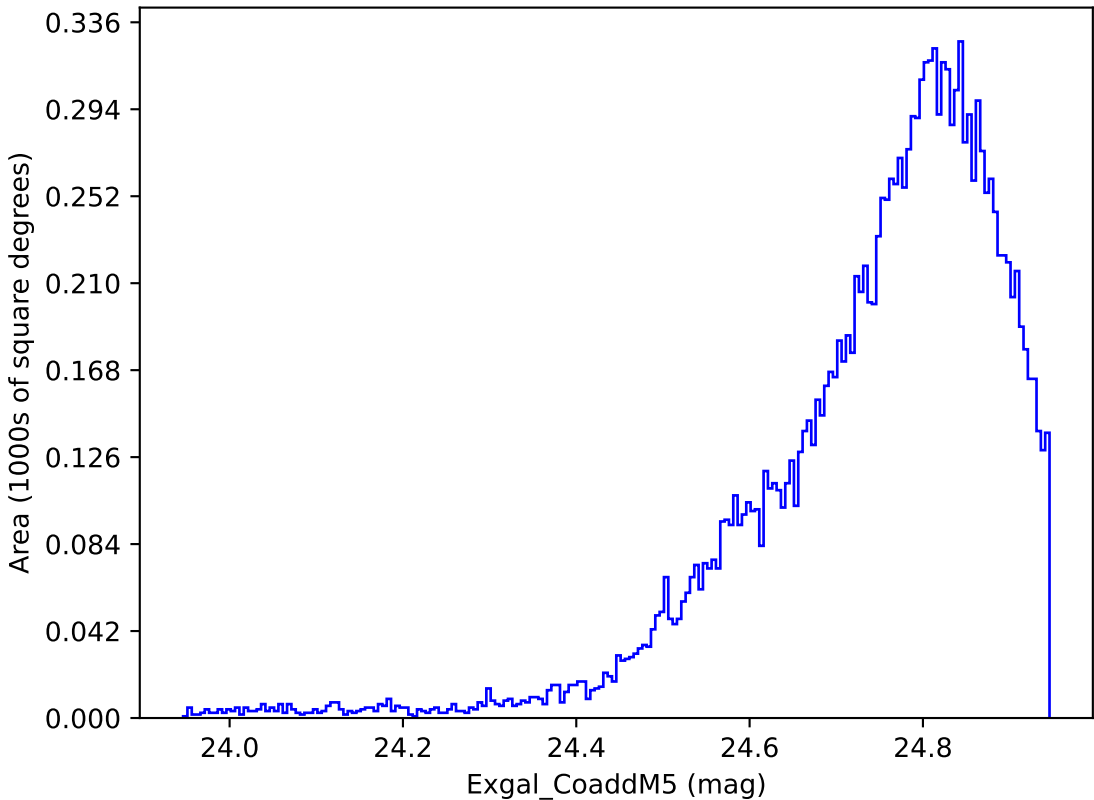
too_elab_r16_d2_giz_v3.4_10yrs WFD y band: Exgal_CoaddM5
