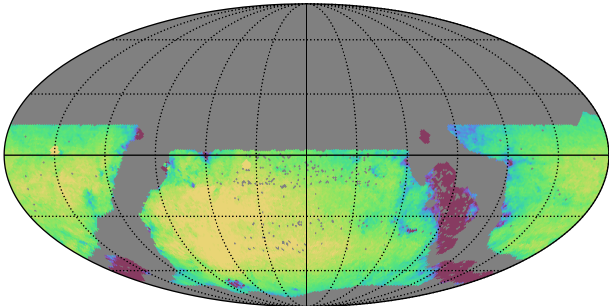
too_elab_r16_d2_giz_v3.4_10yrs WFD r band: Exgal_CoaddM5
