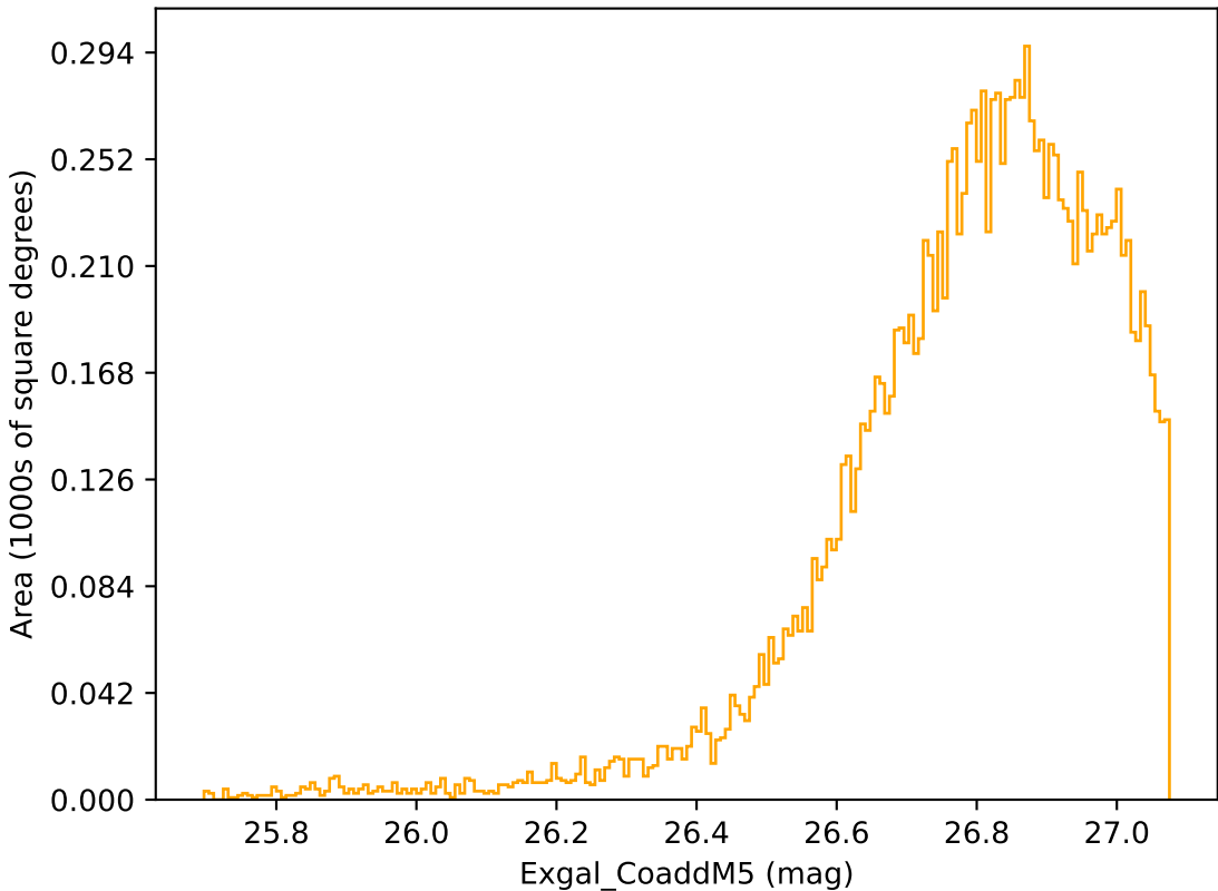
too_elab_r16_d2_giz_v3.4_10yrs WFD r band: Exgal_CoaddM5
