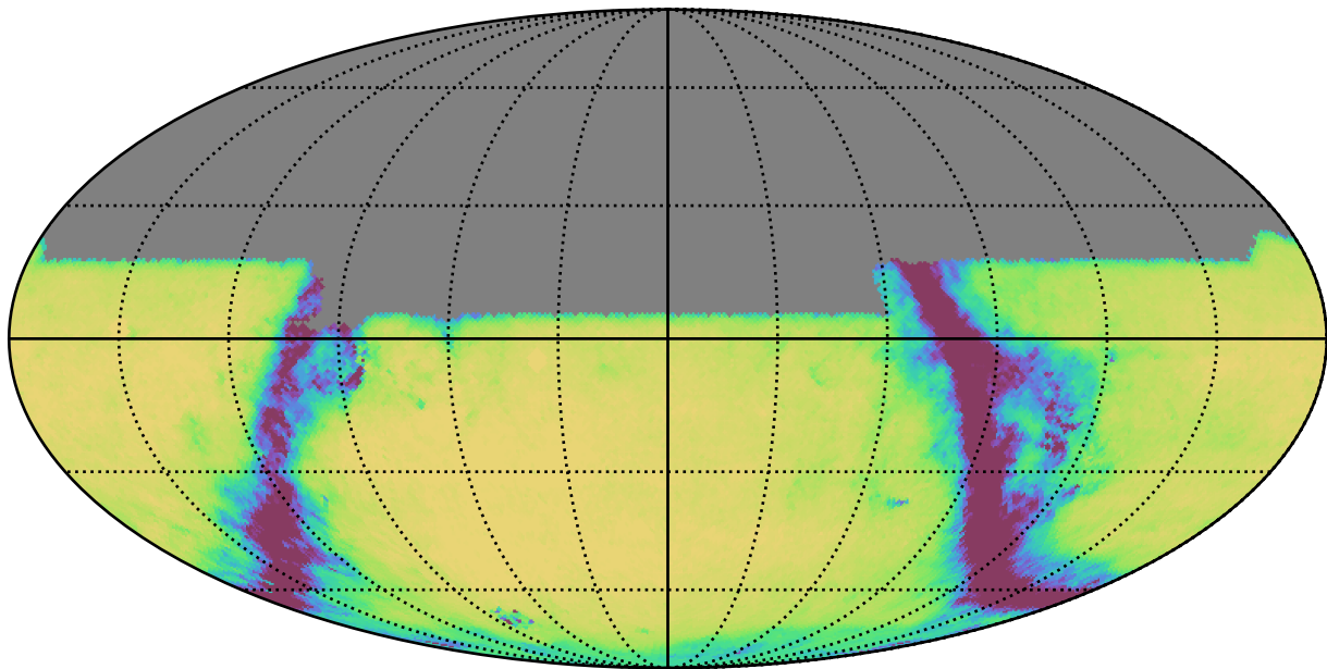
too_elab_r16_d2_giz_v3.4_10yrs All sky u band: Exgal_CoaddM5
