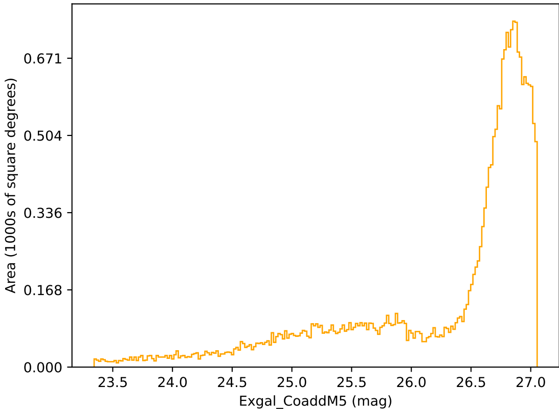
too_elab_r16_d2_giz_v3.4_10yrs All sky r band: Exgal_CoaddM5
