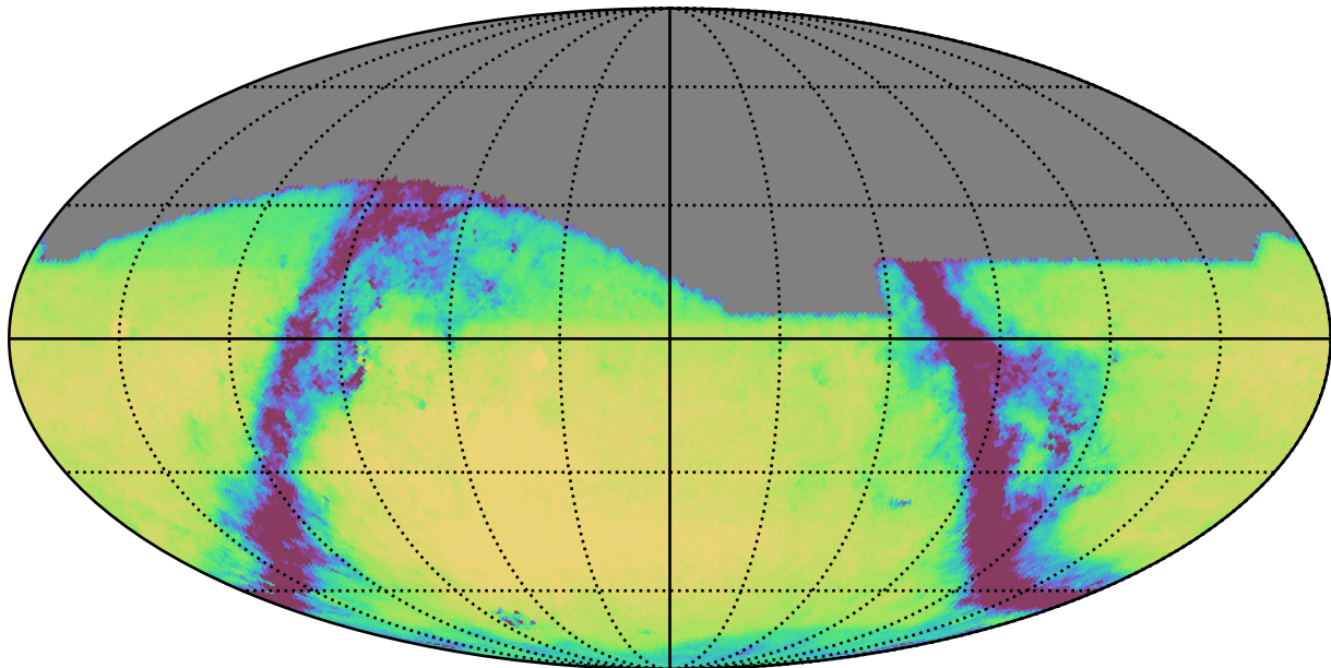
too_elab_r16_d2_giz_v3.4_10yrs All sky g band: Exgal_CoaddM5
