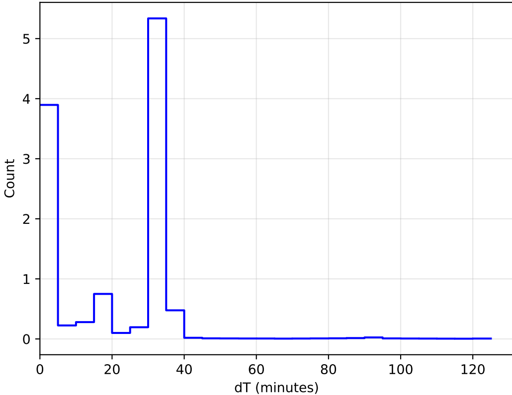
too_elab_r16_d2_giz_v3.4_10yrs WFD: DeltaT Histogram
