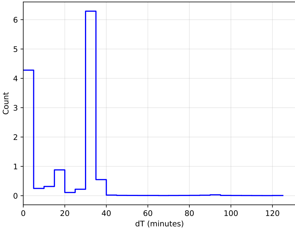
too_elab_r16_d2_giz_v3.4_10yrs All sky: DeltaT Histogram 1e6
