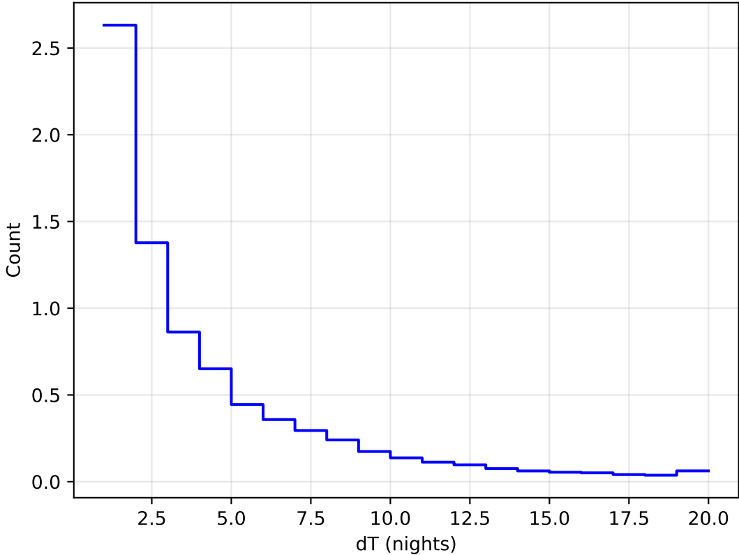
too_elab_r16_d2_giz_v3.4_10yrs WFD all bands: DeltaNight Histogram 1e6
