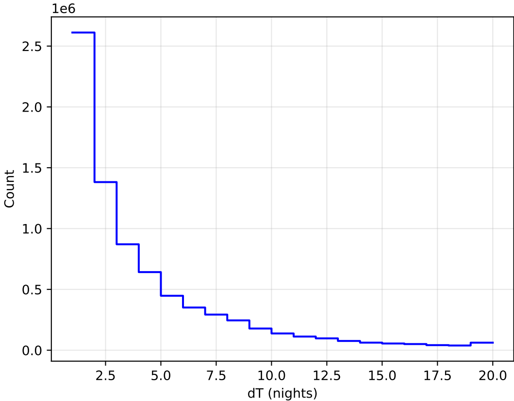
too_elab_r16_d2_giz_v3.4_10yrs WFD all bands: DeltaNight Histogram
