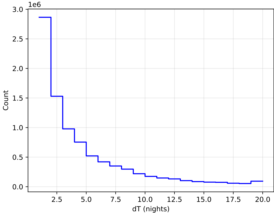
too_elab_r16_d2_giz_v3.4_10yrs All sky all bands: DeltaNight Histogram
