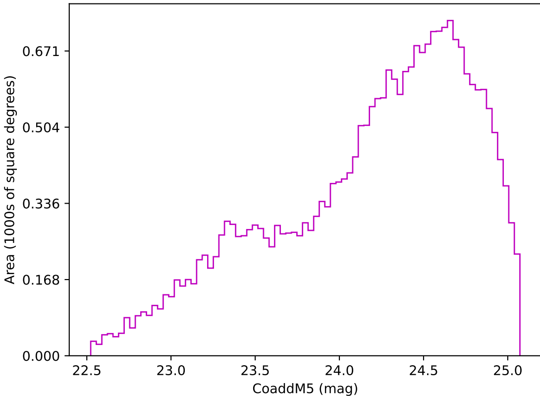
too_elab_r16_d2_giz_v3.4_10yrs Yr 3-4 z band: CoaddM5
