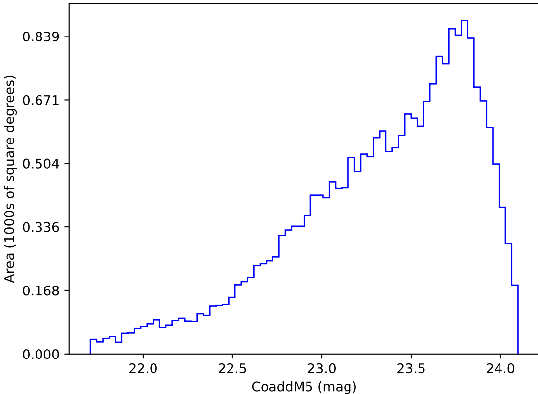
too_elab_r16_d2_giz_v3.4_10yrs Yr 3-4 y band: CoaddM5
