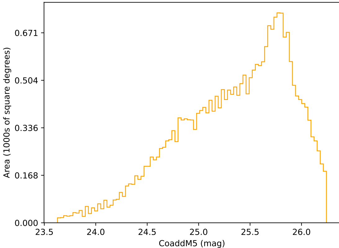
too_elab_r16_d2_giz_v3.4_10yrs Yr 3-4 r band: CoaddM5
