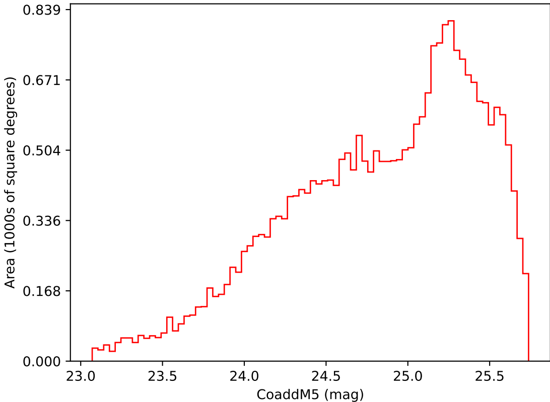
too_elab_r16_d2_giz_v3.4_10yrs Yr 3-4 i band: CoaddM5
