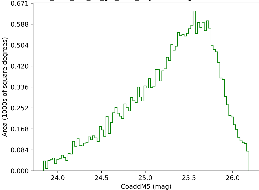
too_elab_r16_d2_giz_v3.4_10yrs Yr 3-4 g band: CoaddM5
