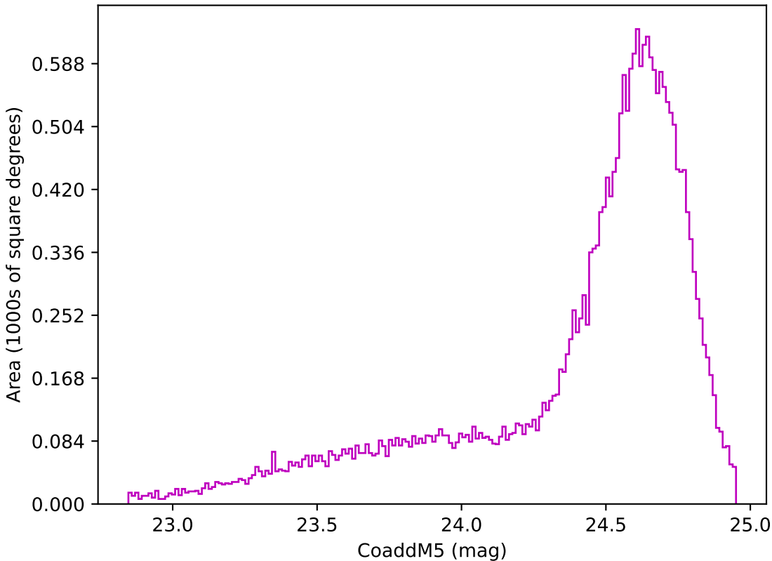
too_elab_r16_d2_giz_v3.4_10yrs Yr 1 z band: CoaddM5
