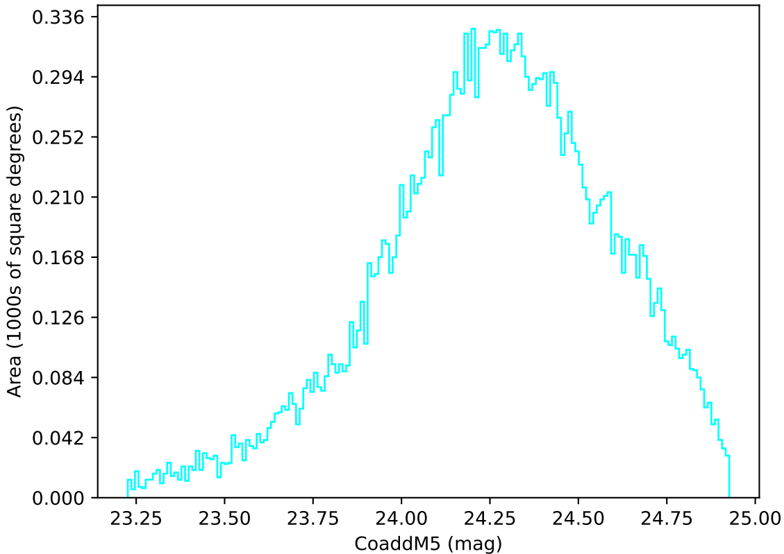
too_elab_r16_d2_giz_v3.4_10yrs Yr 1 u band: CoaddM5
