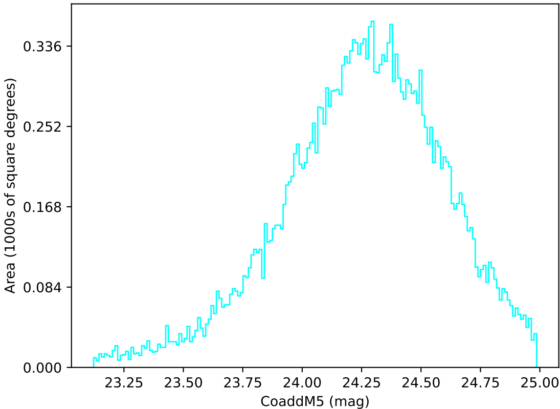
too_elab_r16_d2_giz_v3.4_10yrs Yr 1 u band: CoaddM5
