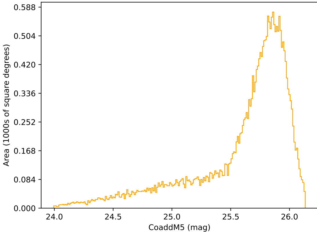
too_elab_r16_d2_giz_v3.4_10yrs Yr 1 r band: CoaddM5
